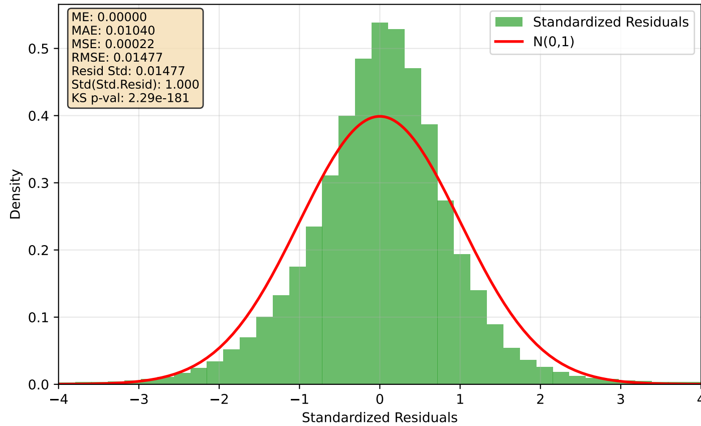
explicit Standardized Residuals
